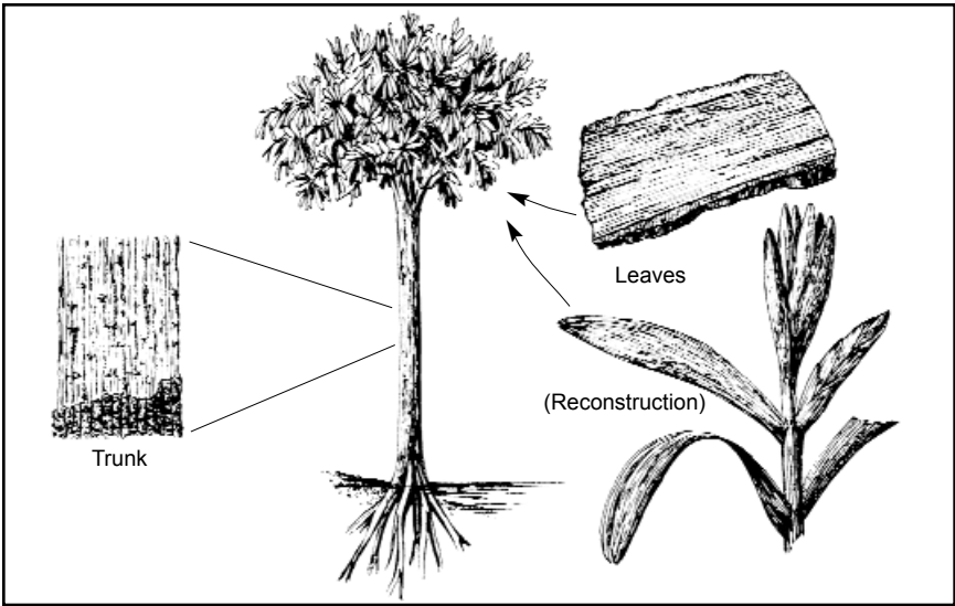
Figure 8. Cordaites , a coal-age tree.
