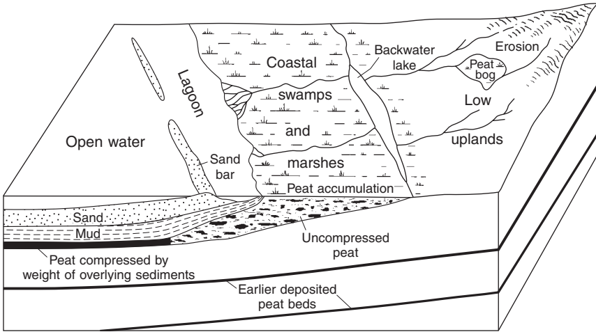
Figure 2. The accumulation of peat in coastal swamps.
