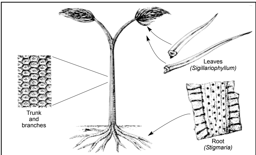
Figure 7. Sigillaria , a coal-age tree.
