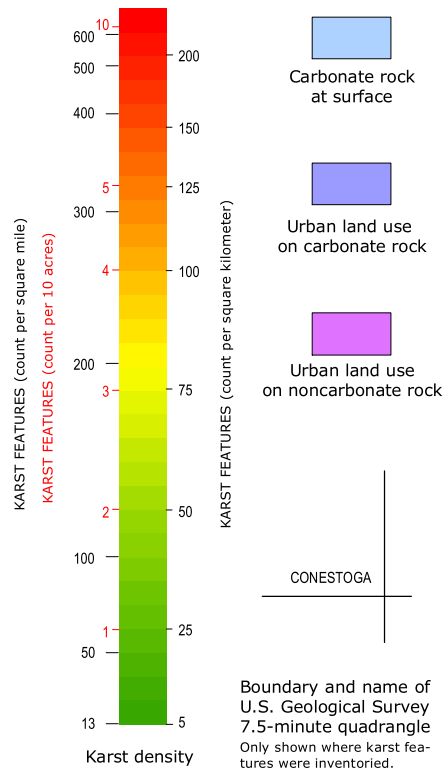
FROM MAP 68: DENSITY OF MAPPED KARST FEATURES IN SOUTH-CENTRAL AND SOUTHEASTERN PENNSYLVANIA
